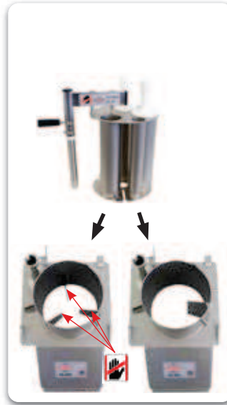
4-TUBE INSERT
